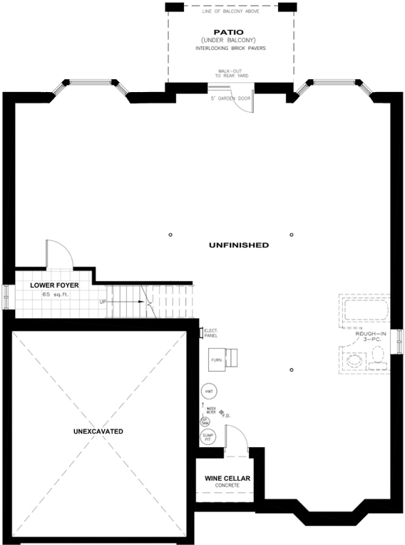
BASEMENT PLAN
