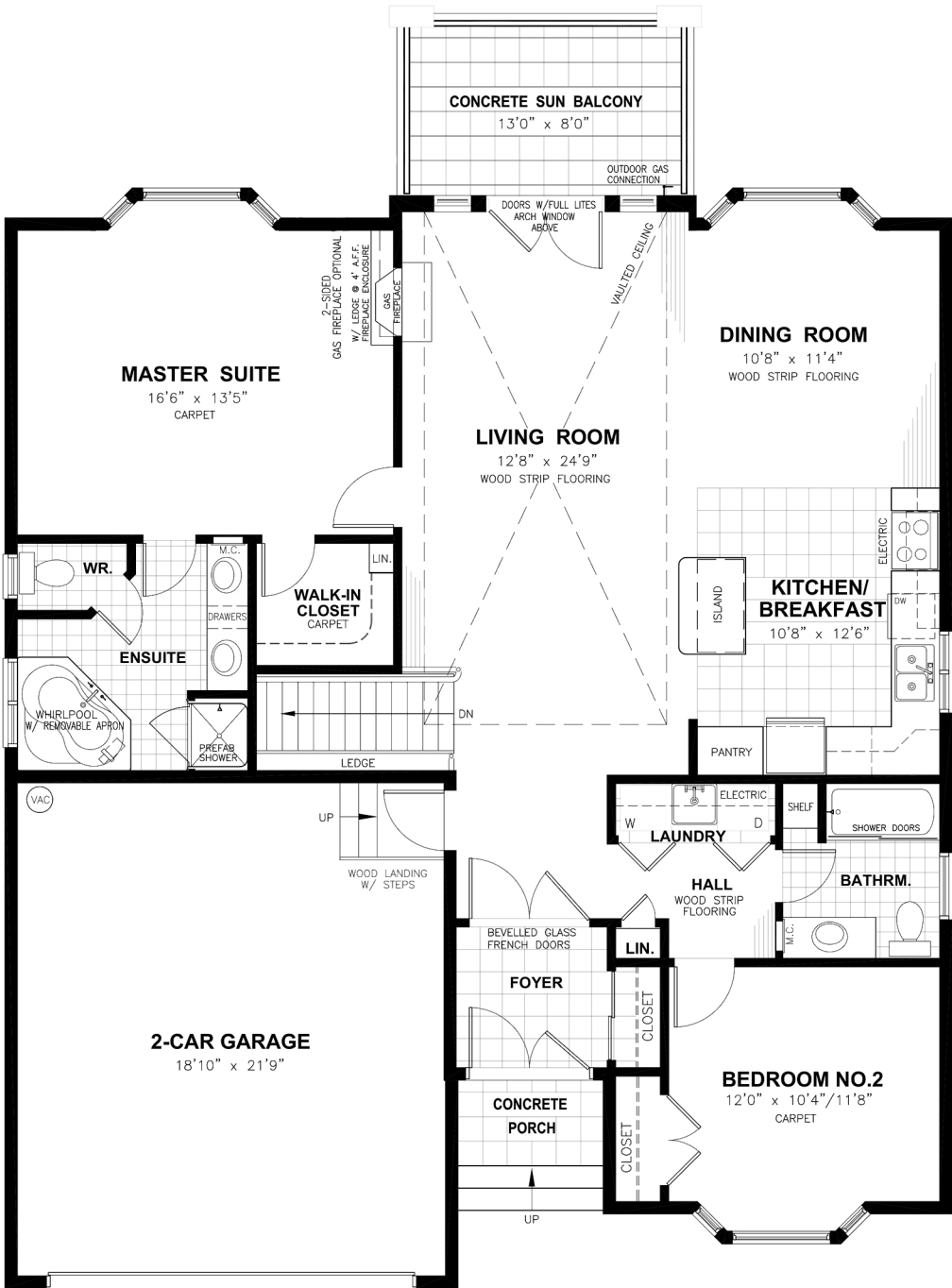
GROUND FLOOR PLAN 1,500 sq.ft.
